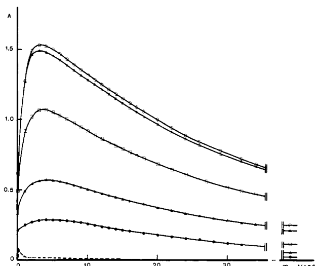
Figure 2. Plots of absorbance at 333 nm (2-cm optical path) vs. time for the reaction of 3.3 \times 10^{-2} \text{ M} cyclohexene with 5.7 \times 10^{-4} \text{ M} bromine in the presence of pyridine in 1,2-dichloroethane at 25 °C: 10^3 [\text{py}] (---) 0; (●) 1.3; (▲) 2.3; (□) 6.6; (△) 29.4; (○) 61.0 M.
