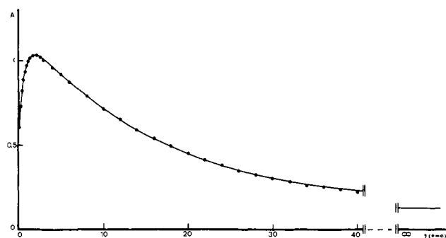
Figure 4. Experimental (—) and calculated (---) plot of absorbance at 350 nm (2-cm optical path) vs. time for the reaction of 4.92 × 10 -4 M bromine with 4.95 × 10 -2 M cyclohexene in the presence of 5.04 × 10 -2 M pyridine in 1,2-dichloroethane at 25 °C (run 26 of Table III).
