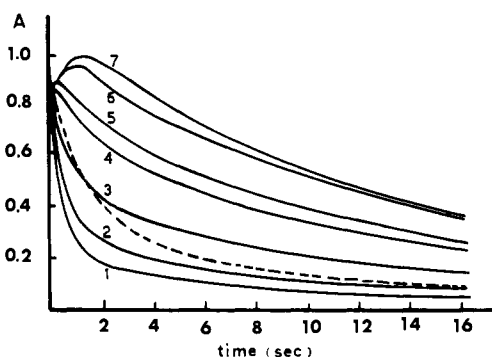
Figure 1. Plots of absorbance at 405 nm (2-cm optical path) vs. time for the reaction of 5.0 \times 10^{-2} \text{ M} cyclohexene with 2.3 \times 10^{-3} \text{ M} bromine in the presence of pyridine in 1,2-dichloroethane at 25 °C: 10^3 [\text{py}] (---) 0 (time scale \times 10^2 ); (1) 2.3; (2) 4.1; (3) 8.8; (4) 17.0; (5) 26.0; (6) 45.0; (7) 100.0 M.
